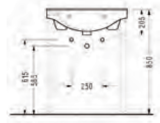
Washbasin With Shelf (85 cm.)
