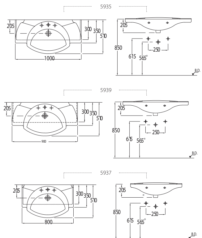
Washbasin With Shelf (90 cm.)
